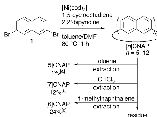
Scheme 1. Synthesis and isolation of [n] CNAP. [a] Yield of isolated product after subsequent purification by GPC. [b] Yield of isolated product after subsequent purification by recrystallization from o -dichlorobenzene. [c] Yield of isolated product after subsequent purification by recrystallization from nitrobenzene. cod = 1,5-cyclooctadiene, DMF = N,N -dimethylformamide.
